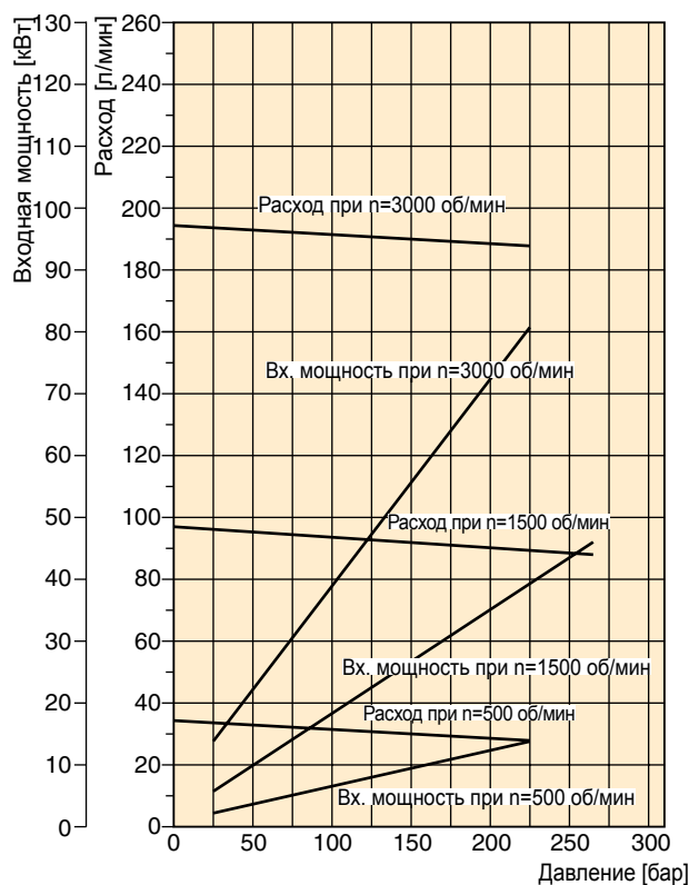
PGP640 - 65,0 см³/об
